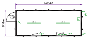
Bungalow bureau 20' standard
