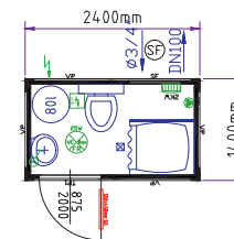
Conteneur WC-douche 8'
