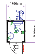
Conteneur WC 5'
